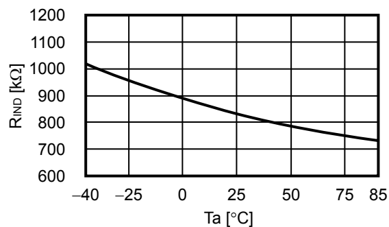
3.5 R_{INI1} - T_a
