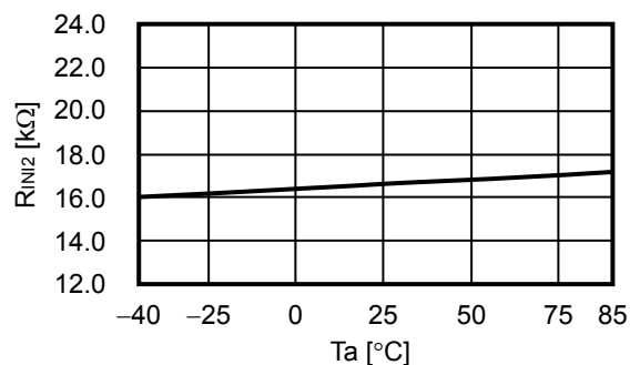
3.7 R_{INI2} - T_a
